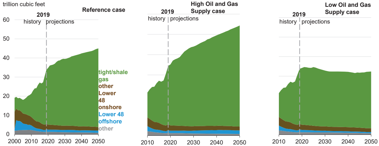
AEO2020 dry natural gas production by type trillion cubic feet
