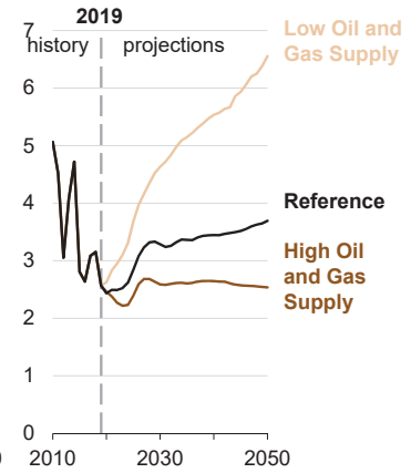
Natural gas price at Henry Hub
