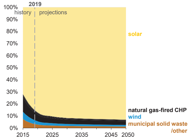
Commercial distributed generation capacity (AEO2020 Reference case) percent
